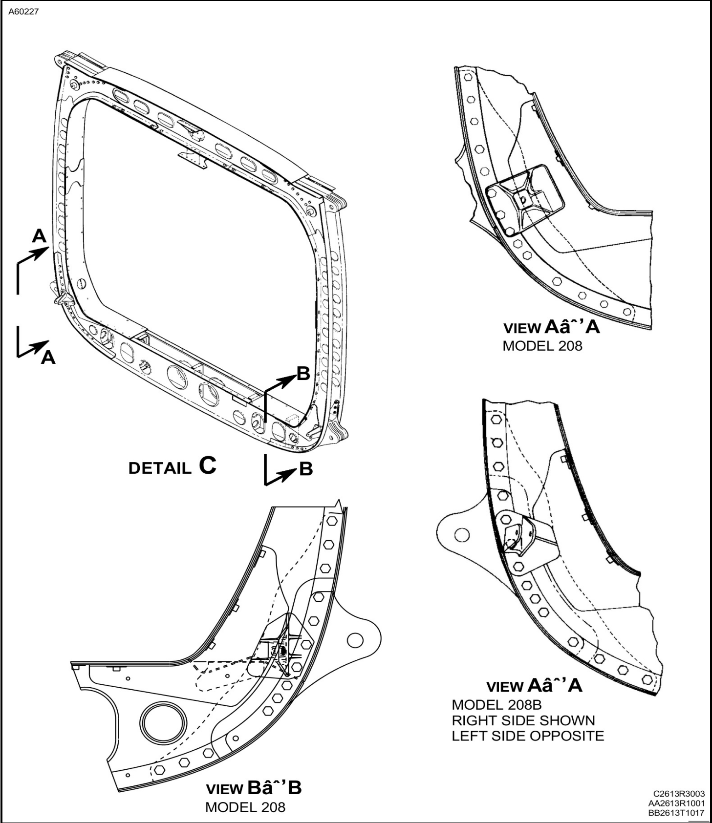
Figure 201 : Sheet 2 : Bolt Identification
