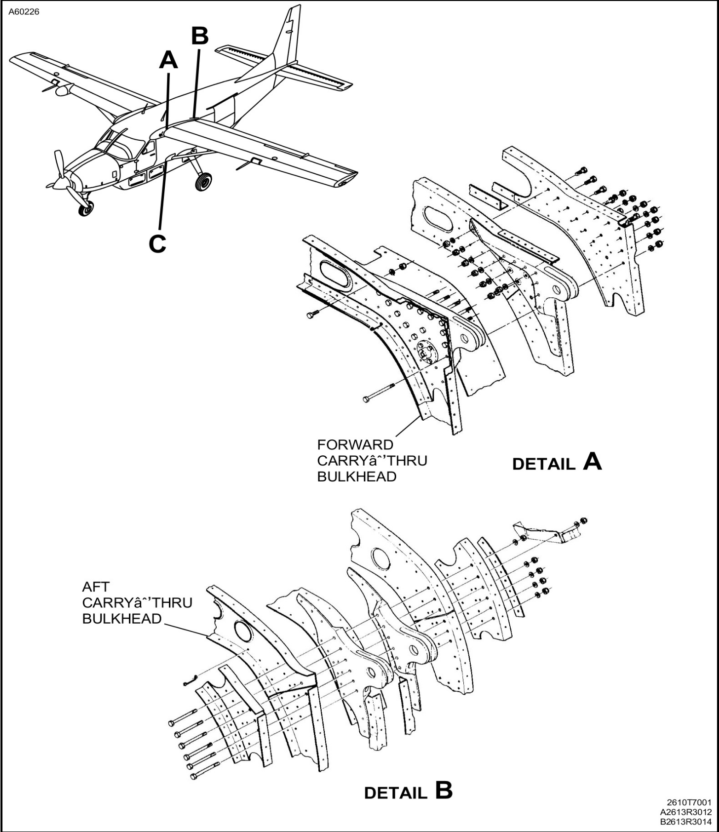
Figure 201 : Sheet 1 : Bolt Identification
